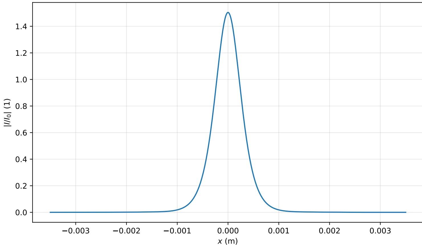
Intensity profile I(x, y = 0, z = 3.423m)/I_0 , P_{in}=0.9P_{cr} , artificial time
